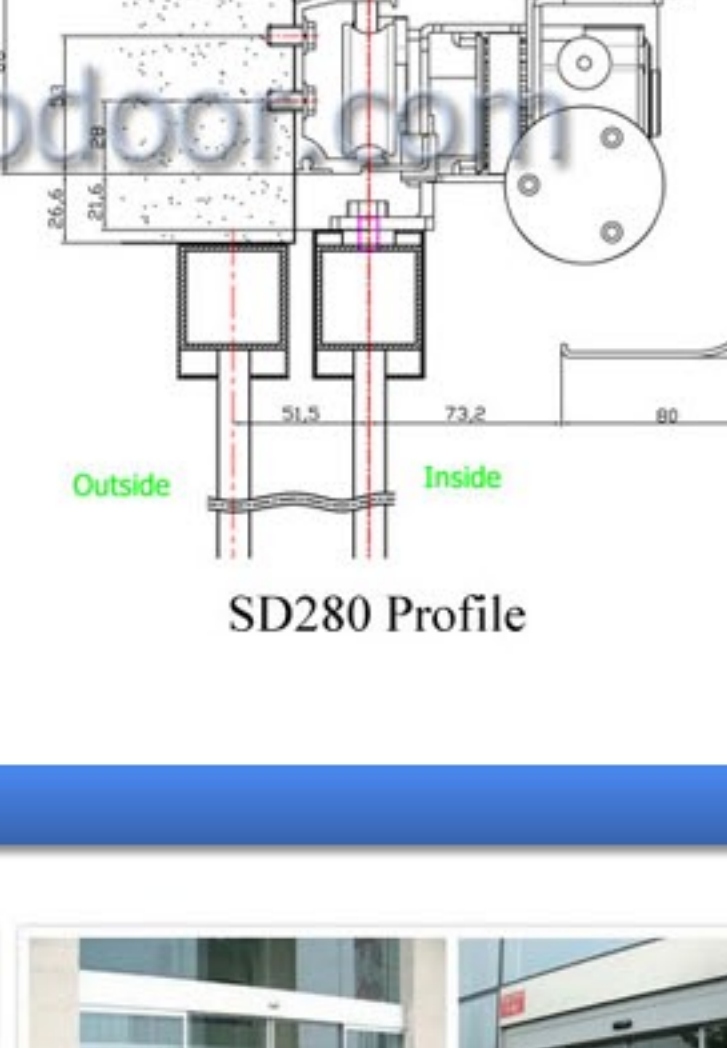
SD280 Profile
