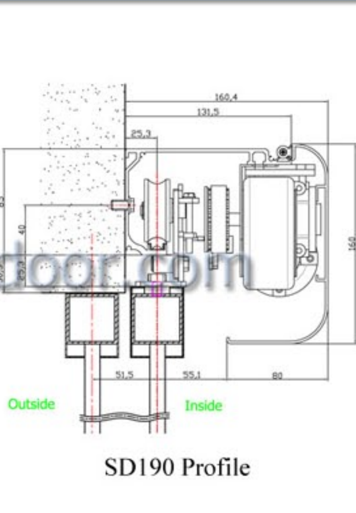
SD190 Profile
