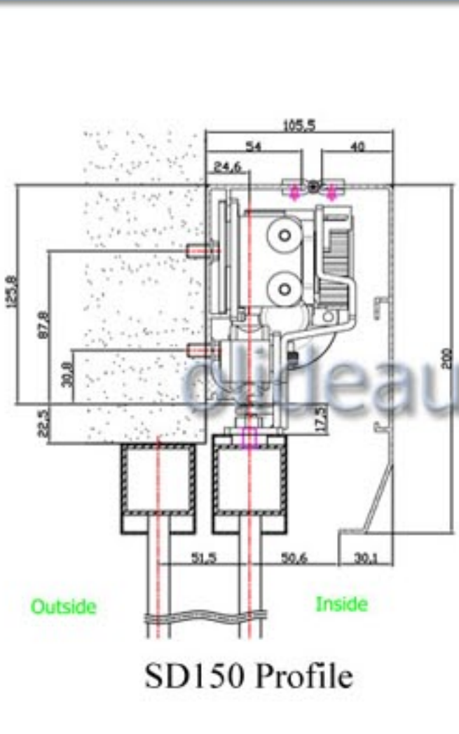
SD150 Profile
